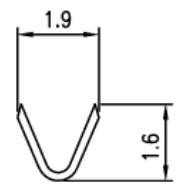
B-B SECTION
