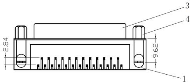
Jack Screws & Board Locks (06)
