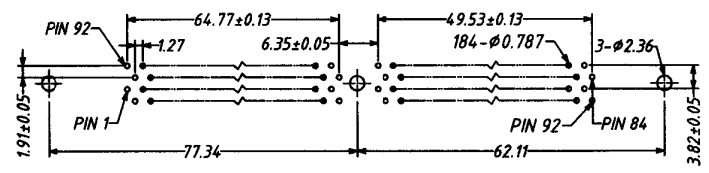
PC Board Layout
