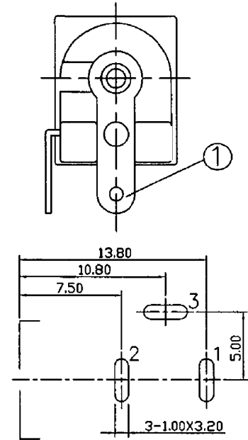
Pin Hole Layout (Jack Bottom View)
