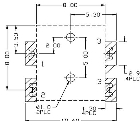
Recommended PAD Layout (Top View)
