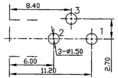
Pin Hole Jack (Jack Bottom View)
