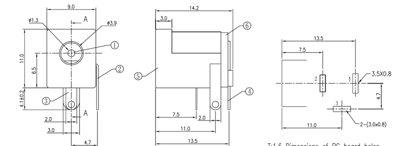
T:1.6 Dimensions of PC board holes Tolerance : ±0.05(Printed-top view)
