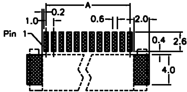
P.C. Board Layout S.M.D. Type (Top View)
