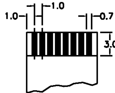
FFC/FPC Dimension Thickness 0.3±0.05mm
