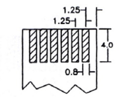
FFC/FPC Dimension Thickness 0.3 \pm 0.05 mm
