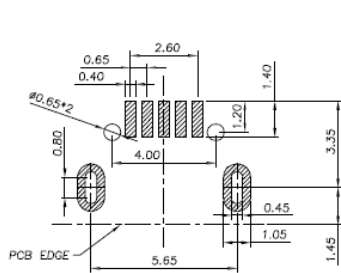
RECOMMENDED PCB LAYOUT (TOL:±0.05)
