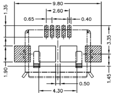
P.C.B. LAYOUT TOP VIEW ±0.05
