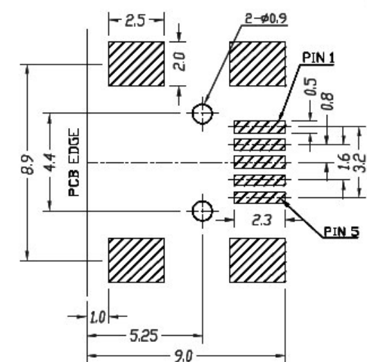
RECOMMENDED PCB PATTERN LAYOUT (PCB THICKNESS 0.8±0.1)
