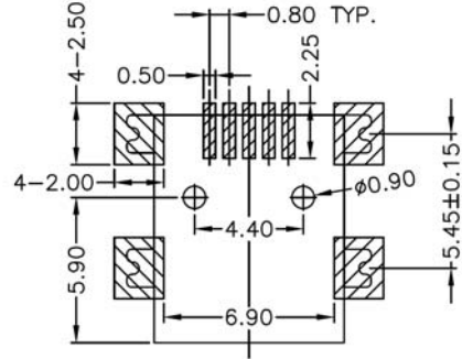
P.C.B. LAYOUT TOP VIEW ±0.05
