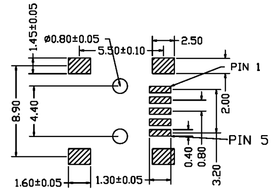
PC Board Layout (Component Side)
