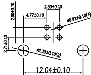
RECOMMENDED P.C.B. PATTERN LAYOUT
