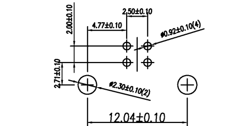
RECOMMENDED P.C.B. PATTERN LAYOUT
