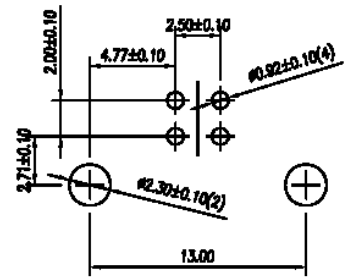
RECOMMENDED P.C.B. PATTERN LAYOUT
