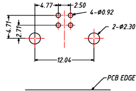
RECOMMENDED P.C.B. PATTERN LAYOUT
