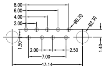
PCB LAYOUT TOLERANCE: ±0.05
