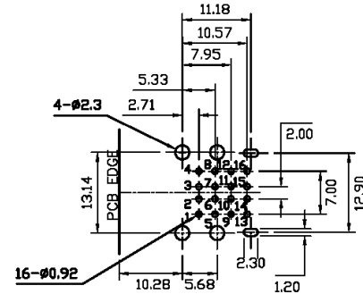
BOTTOM VIEW RECOMMENDED PCB LAYOUT A
