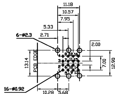
BOTTOM VIEW RECOMMENDED PCB LAYOUT B
