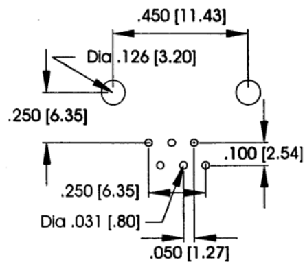
6P4C - 6P6C
