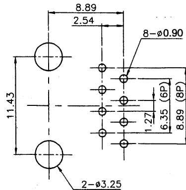
PC Board Layout (Top View)
