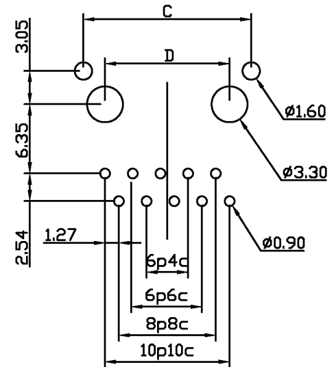
PC Board Layout (Top View)
