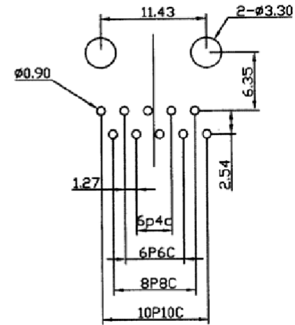
PC Board Layout (Top View)
