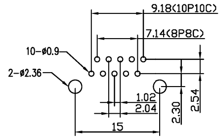
LAYOUT/TOP VIEW
