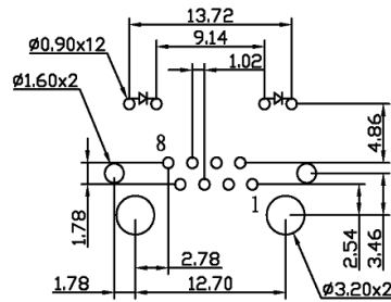
PC BOARD LAYOUT/TOP VIEW
