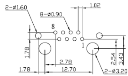
PC BOARD LAYOUT/TOP VIEW
