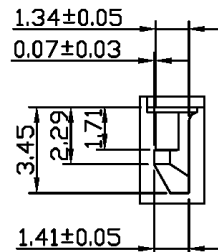
DETAIL X
