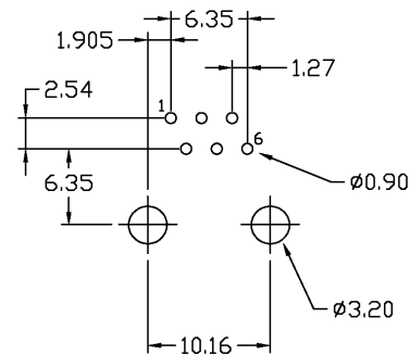
PC Board Layout Ref.
