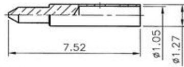
SOLDER CONTACT PIN
