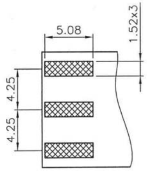
RECOMMENDED MOUNTING PATTERN 1. MAX. PANEL THICKNESS=10
