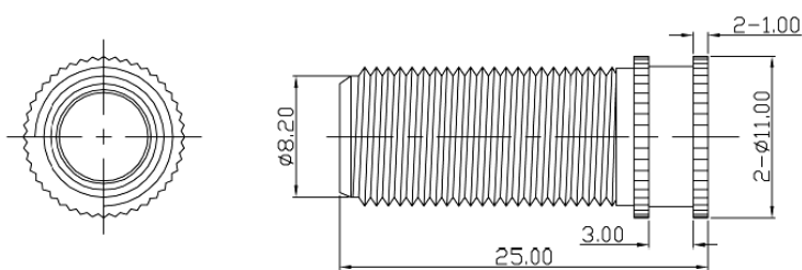
F-CONN. W/PIN1-BODY
