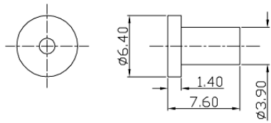
F-CONN. W/PIN1-INSULATOR
