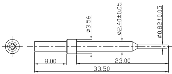
F-CONN. W/PIN1- PIN
