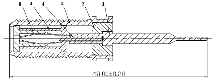
(Assembly)
