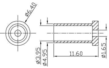
F-CONN. W/PIN1-COVER
