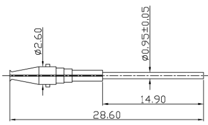
F-CONN. W/PIN1-RECEPTER
