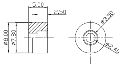
F-CONN. PIN1-INSULATOR
