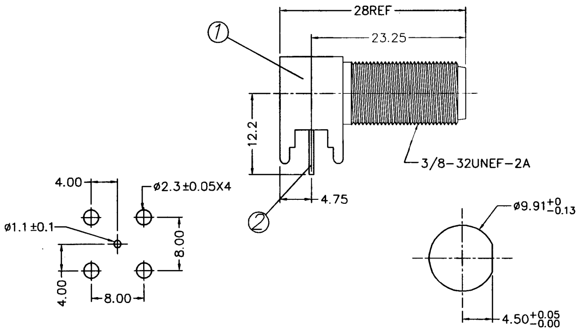
PC Board Hole Configuration
