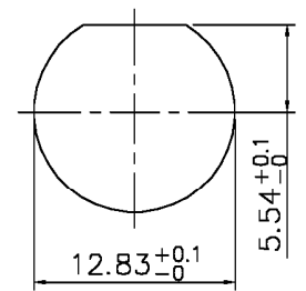
Recommended Mounting Hole (Maximum Panel Thickness: 5.5mm)
