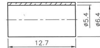
RECOMMENDED CABLE STRIPPING DIM'S (建議剝線尺寸)
