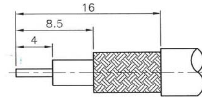
RECOMMENDED CABLE STRIPPING DIM'S (建議剝線尺寸)
