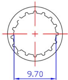
④ LOCK WASHER
