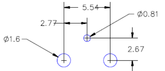
SUGGESTED MOUNTING HOLE PATTERN
