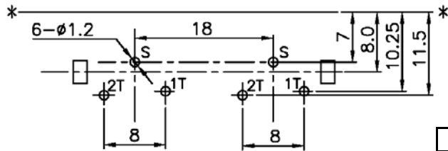
PCB Hole Dimensions ±0.1 (Printed-top view)
