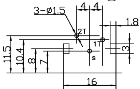
PCB Hole Dimensions ±0.1 (Printed-top view)
