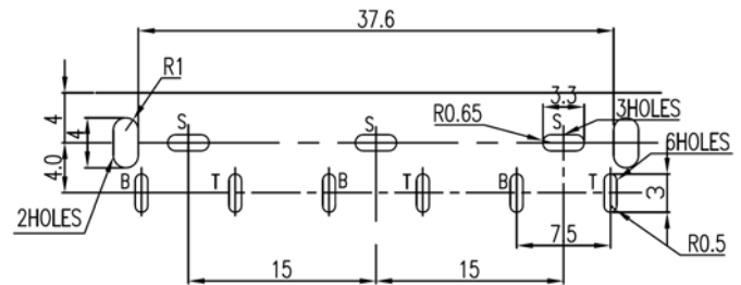
T:1.6 Dimensions of PC board holes Tolerance : ±0.1(Printed-top view)
