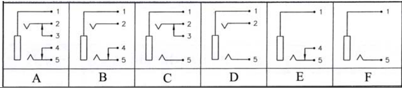
Schematic
