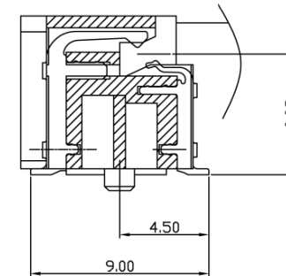
B-B' SECTION
