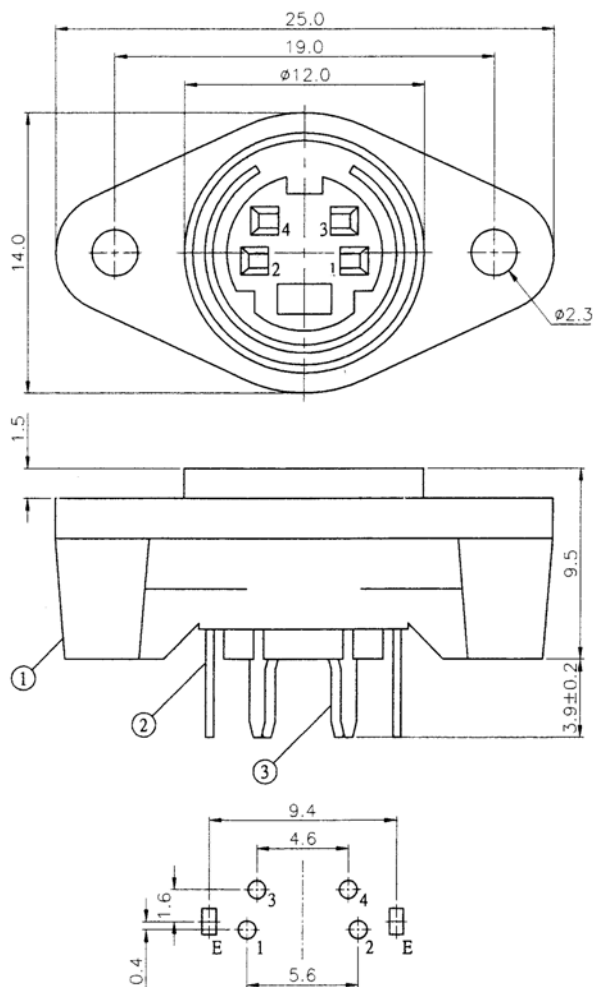
HOLE LAYOUT BOTTOM VIEW
