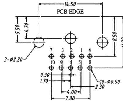
P.C.B. RECOMMEND LAYOUT (BOTTOM VIEW)
