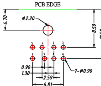
P.C.B. RECOMMEND LAYOUT (BOTTOM VIEW)
