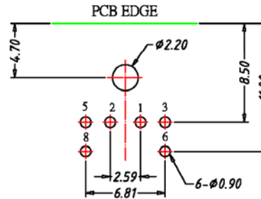
P.C.B. RECOMMEND LAYOUT (BOTTOM VIEW)
