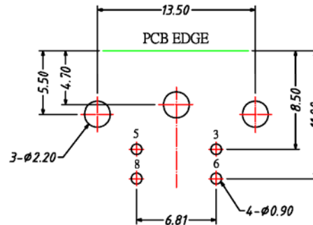
P.C.B. RECOMMEND LAYOUT (BOTTOM VIEW)
