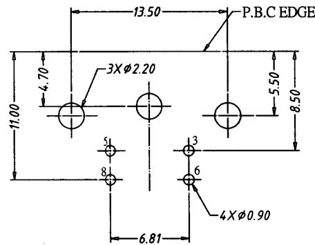
P.C.B. RECOMMEND LAYOUT (BOTTOM VIEW)
