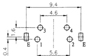
HOLE LAYOUT BOTTOM VIEW
