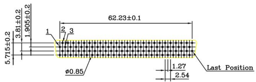
PCB Layout (B)
